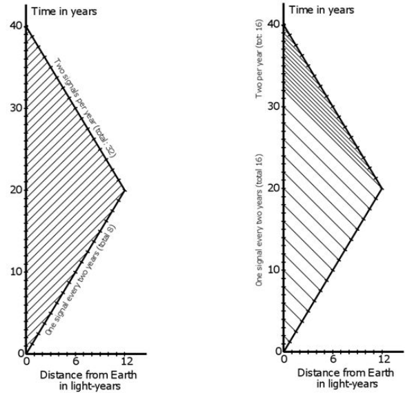
(a) Adelle receives the signal from Chris' flashing clock.
