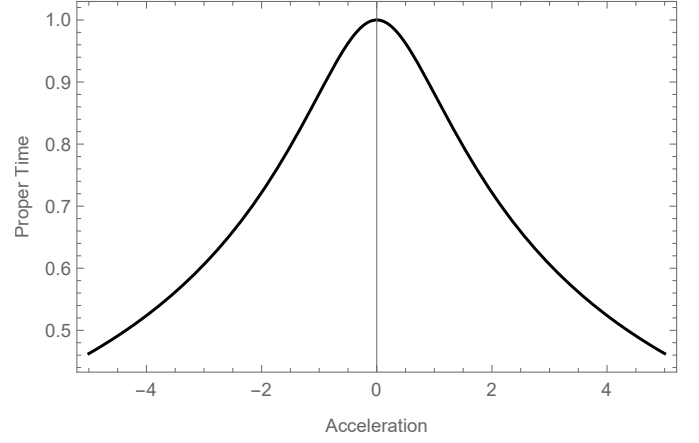
Figure 3: The proper time \Delta\tau of a uniformly accelerated observer as a function of acceleration g assuming \Delta t = c = 1 .
