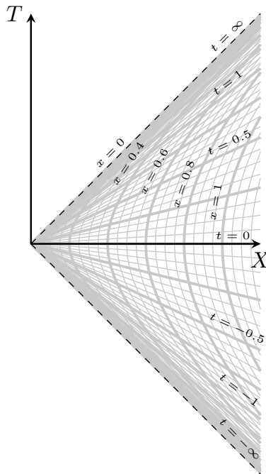
Figure 4: The Rindler coordinate chart otherwise known as the Rindler wedge. It demonstrates lines of simultaneity in Rindler coordinates [13].
